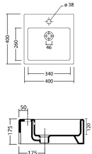
ISA 40 X 40 FINE FIRECLAY WALL HUNG WASH BASIN
