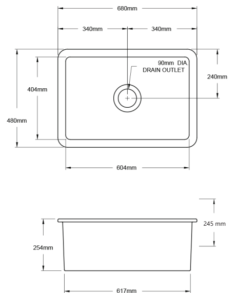
CUISINE 48 X 68 INSET/UNDERMOUNT FINE FIRECLAY SINK
