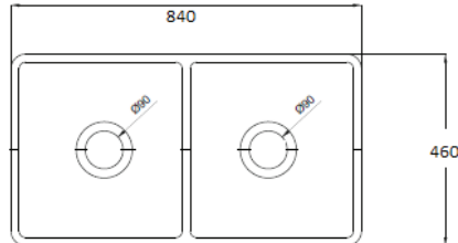
NOVI 84 X 46 FINE FIRECLAY DOUBLE BUTLER SINK
