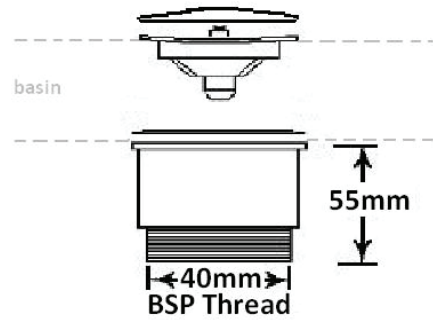
UNIVERSAL 32/40MM TWO PIECE MUSHROOM BRASS POP-UP WASTE
