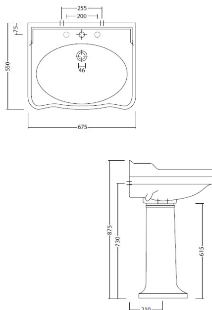
MCKINLEY 70 X 55 FINE FIRECLAY WASH BASIN
