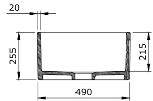
CUISINE 48 X 68 INSET/UNDERMOUNT FINE FIRECLAY SINK
