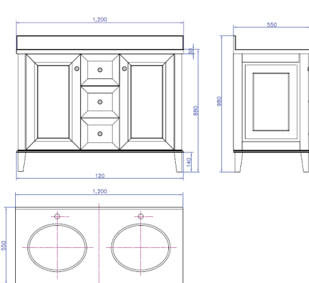
COVENTRY 120 X 55 DOUBLE BOWL SATIN WHITE VANITY WITH REAL MARBLE TOP & CERAMIC UNDERCOUNTER BASIN
