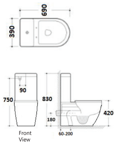
BELMONT CLOSE COUPLED BACK TO WALL TOILET SUITE WITH SOFT CLOSE QUICK RELEASE SEAT
