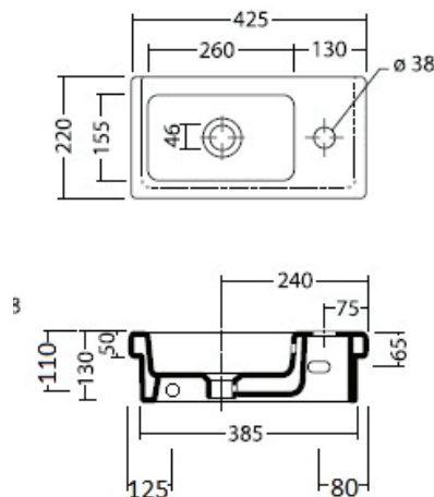
KENYA 42 X 22 FINE FIRECLAY WALL HUNG WASH BASIN
