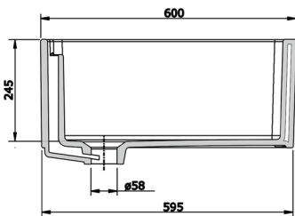
BELFAST 50 X 50 FINE FIRECLAY BUTLER SINK
