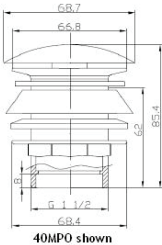
40MM MUSHROOM BATH POP-UP WASTE- NO OVERFLOW
