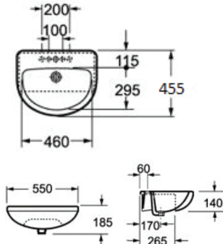
KARIA 55 X 45 SEMI RECESSED CERAMIC WASH BASIN
