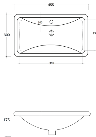
PYRENEES 46 X 30 UNDER COUNTER CERAMIC WASH BASIN
