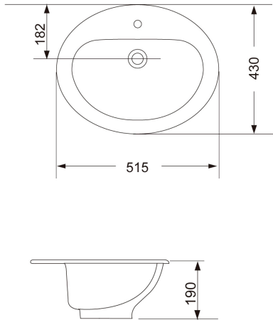
LEON 51 X 43 INSET CERAMIC WASH BASIN
