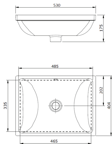
BIAR 52 X 39 UNDER COUNTER CERAMIC WASH BASIN
