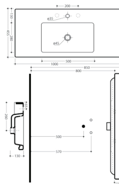
CANGAS 100 X 45 FINE FIRECLAY WASH BASIN
