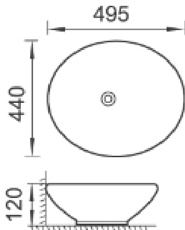
NARVA 50 X 44 COUNTER TOP CERAMIC WASH BASIN
