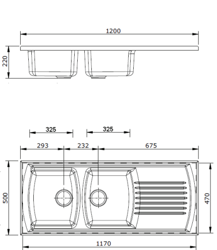
LUSITANO 120 X 50 RECESSED FINE FIRECLAY KITCHEN SINK
