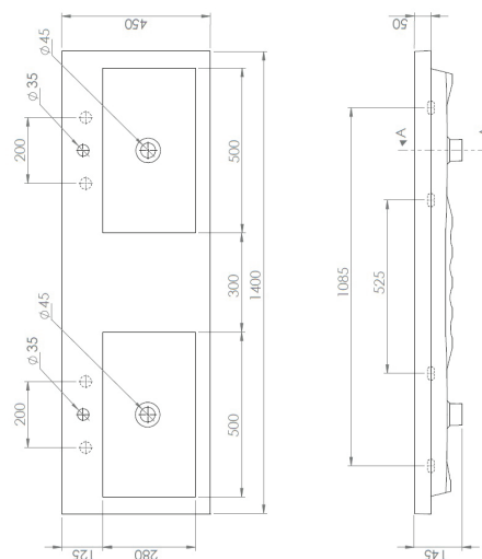
CANGAS 140 X 45 DOUBLE BOWL FINE FIRECLAY WASH BASIN
