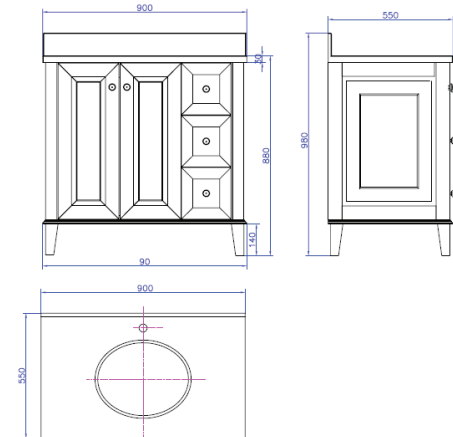
COVENTRY 90 X 55 SATIN WHITE VANITY WITH REAL MARBLE TOP & CERAMIC UNDERCOUNTER BASIN
