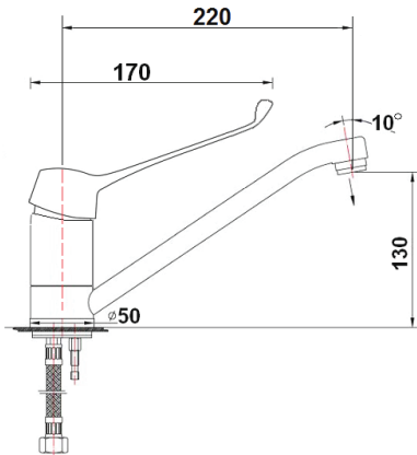
GEORGIA CARE SINK MIXER
