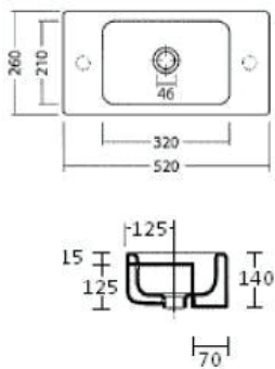
ISA 52 X 26 SEMI RECESSED FINE FIRECLAY BASIN
