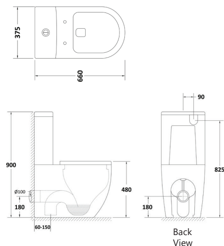
MARSHALL COMFORT HEIGHT CLOSE COUPLED BACK TO WALL TOILET SUITE WITH SOFT CLOSE QUICK RELEASE SEAT
