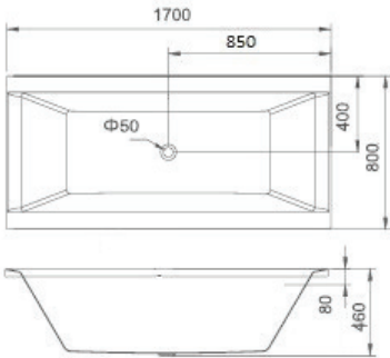
ANZIO 1700 INSET LUCITE ACRYLIC BATH WITH OVERFLOW
