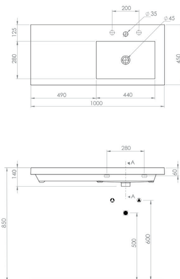
CONDAL 100 X 45 FINE FIRECLAY WASH BASIN
